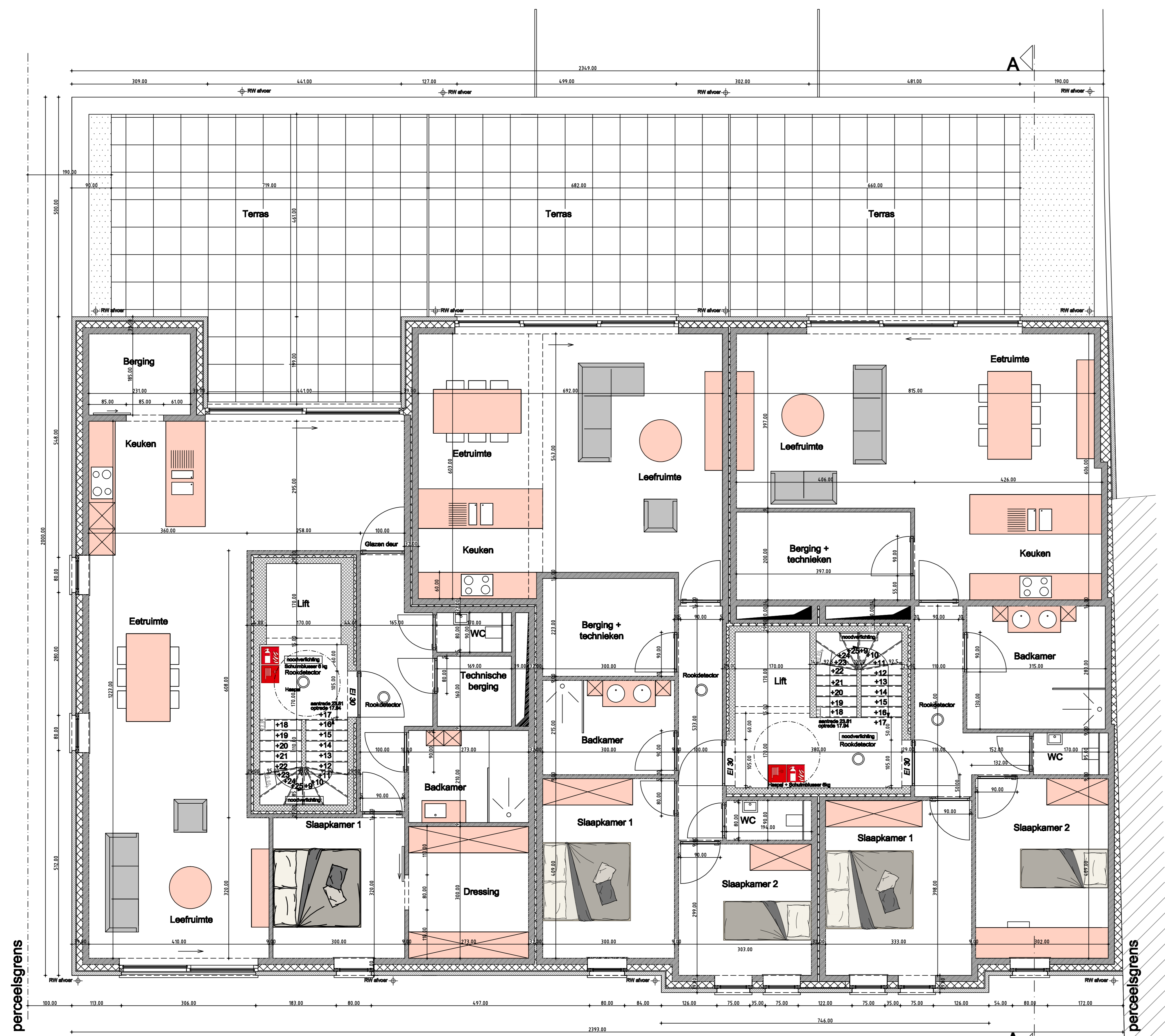
appartement 4 : 1 slaapkamer appartement verdieping +1 schaal 1/50 opp. 115.63 m2 terras opp. 41.70 m2
